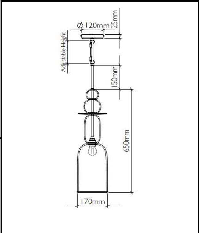
Dimension diagram
